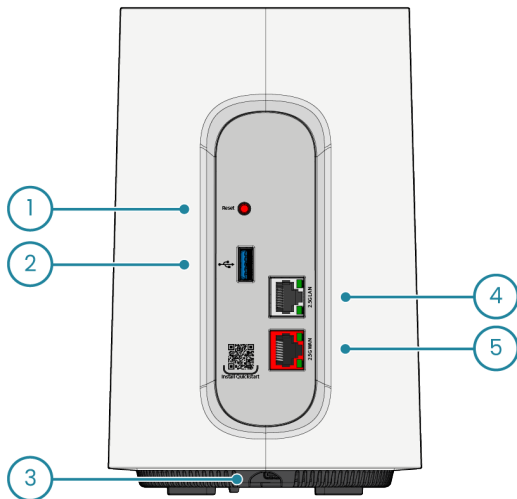
Figure 2: SDG-8622 – Rear View
