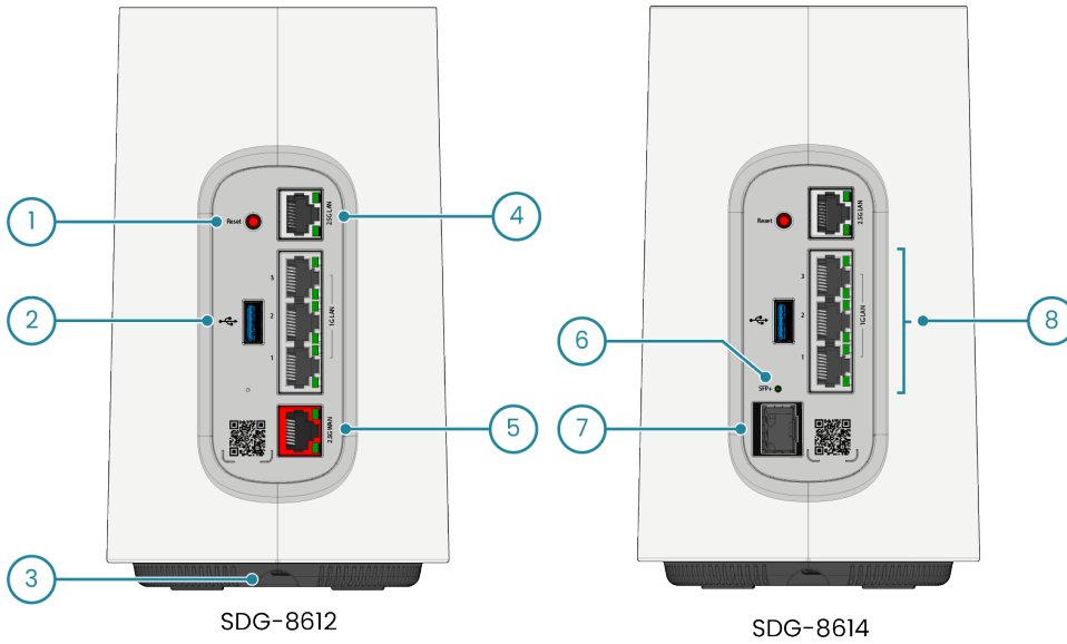
Figure 2: SDG-8612 and SDG-8614— Rear View
